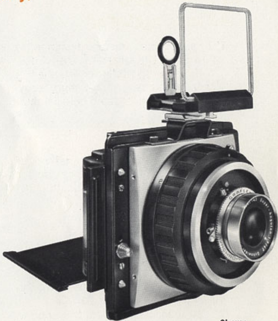
Shown: xlsw camera with lens, sportsfinder, film holder and Graflok® back.
